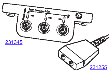
Figure 1. Typical earth bonding points.
