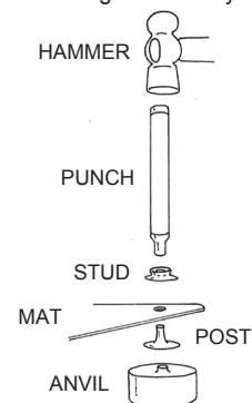
Figure 10. Using the 230660 Punch and Anvil.
